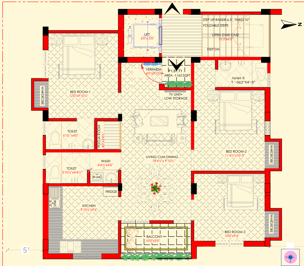
Typical Floor Plan : F1, S1 & T1
