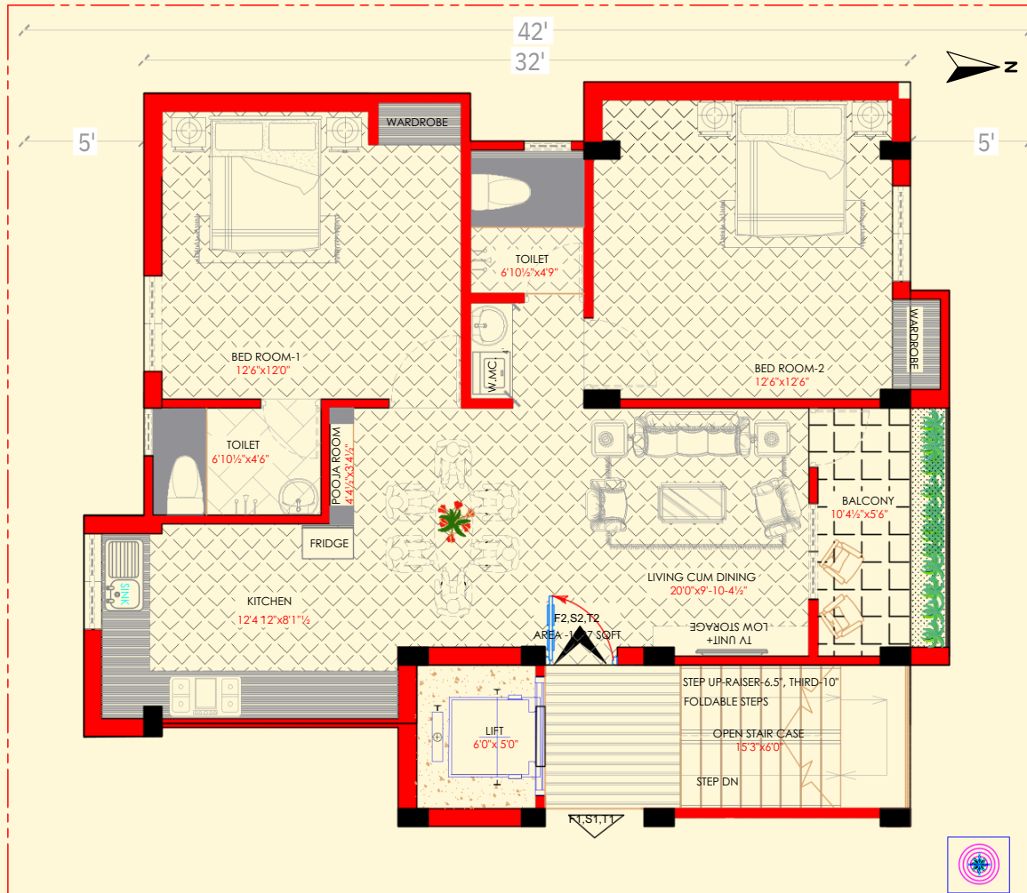
Typical Floor Plan : F2, S2 & T2
